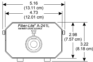
Front Panel Detail
