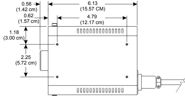
Bottom View with Feet Removed View Showing Four (4) #6-32 Mounting Positions
