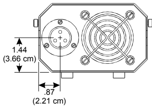
Rear Panel Detail
