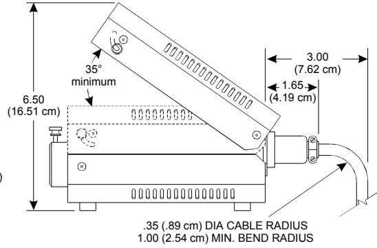
Side Panel Detail
